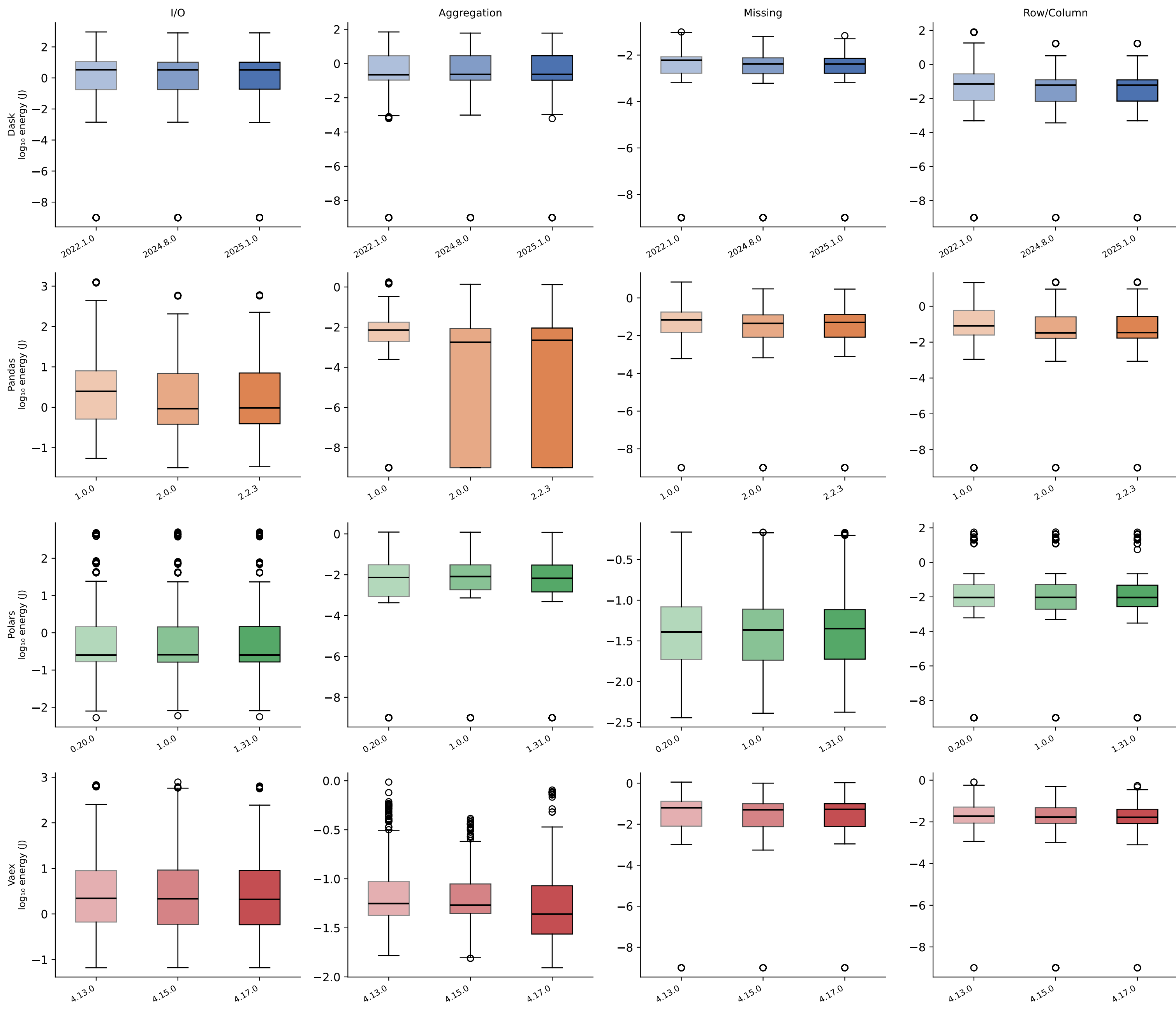
Energy Distribution per Library Version &amp; Operation Category (itr=20)
