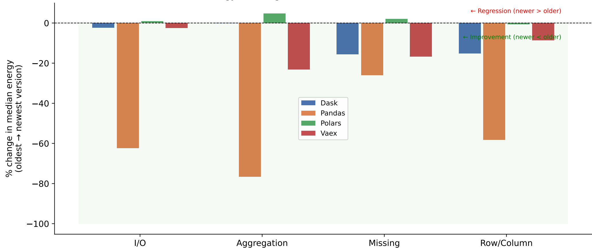
RQ5: Energy % Change from Oldest to Newest Version (itr=30)
