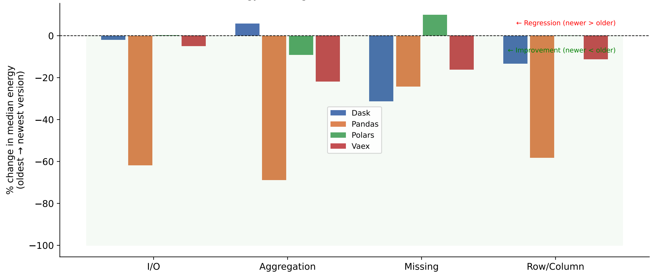
RQ5: Energy % Change from Oldest to Newest Version (itr=20)
