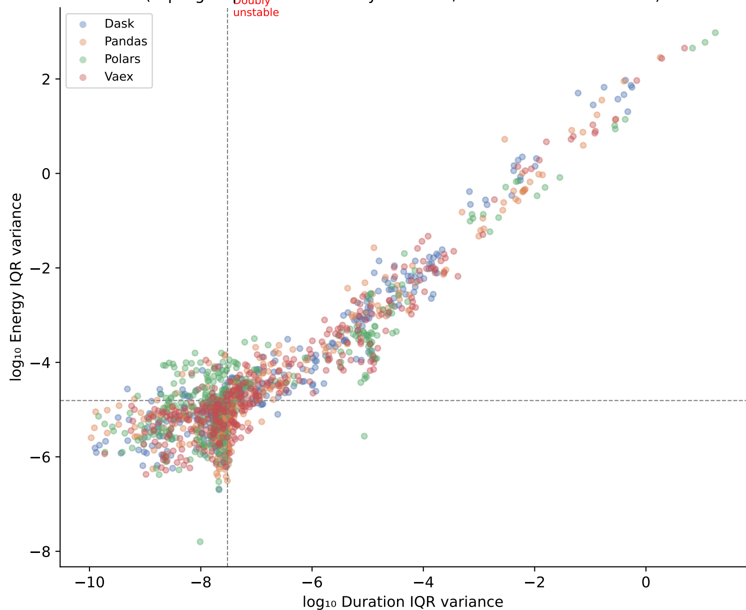
Figure 16 — Energy Variance vs Duration Variance per Function (Top-right quadrant = doubly unstable; dashed lines = medians)
