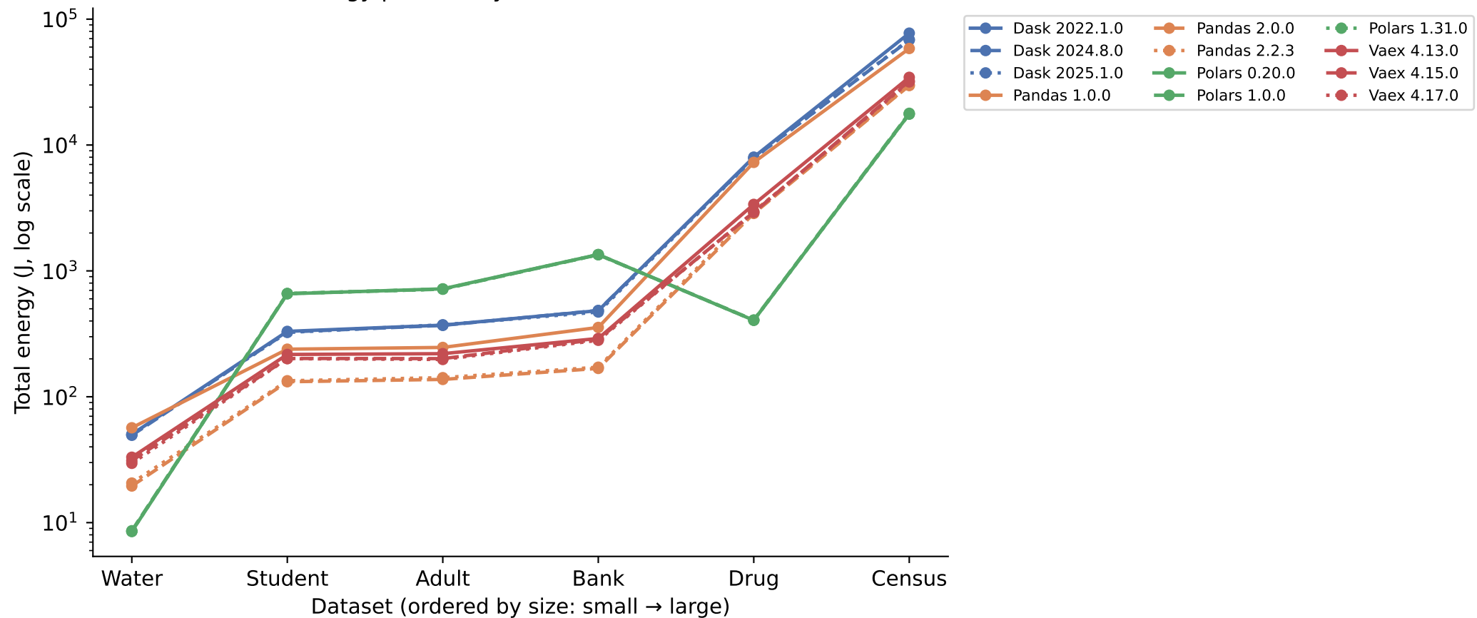
Cumulative Energy per Library Version across Datasets (itr=30)
