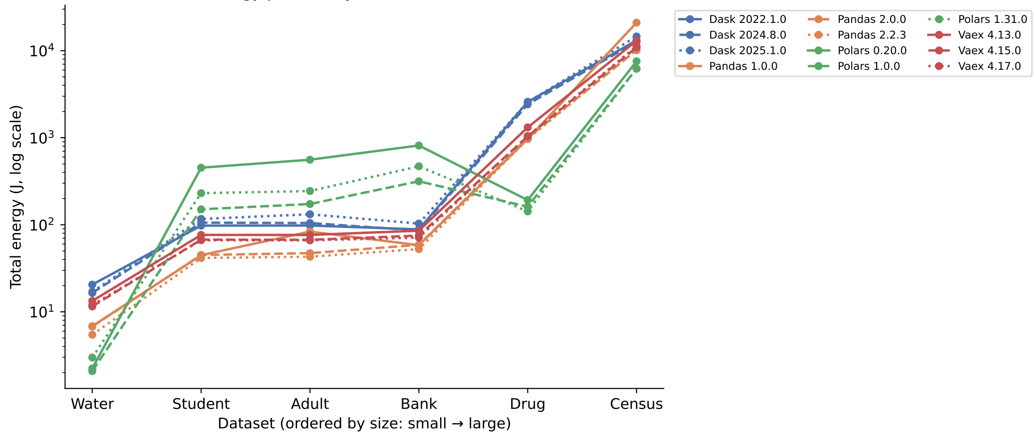
Cumulative Energy per Library Version across Datasets (itr=10)
