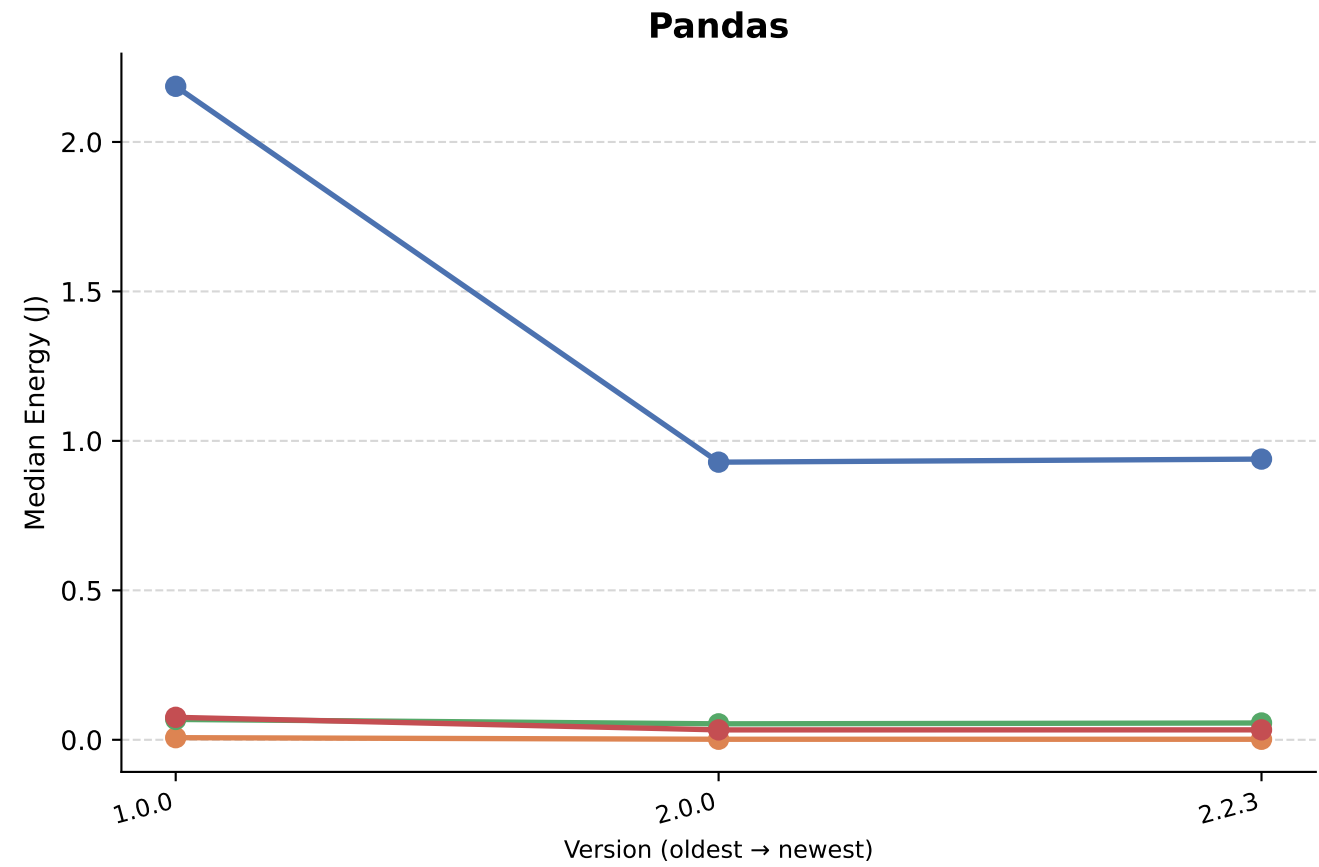
Figure 4: Version Evolution — Median Energy Consumption (Aggregated across datasets and iterations)
