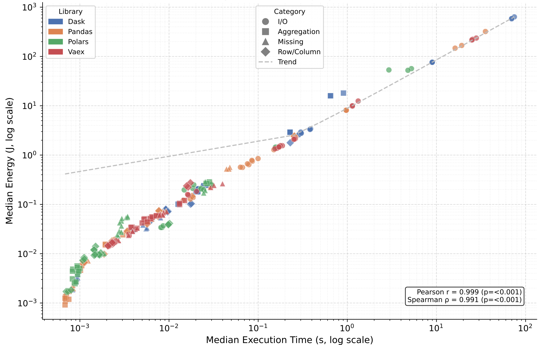
Energy vs Execution Time (per library, version, category, and dataset)
