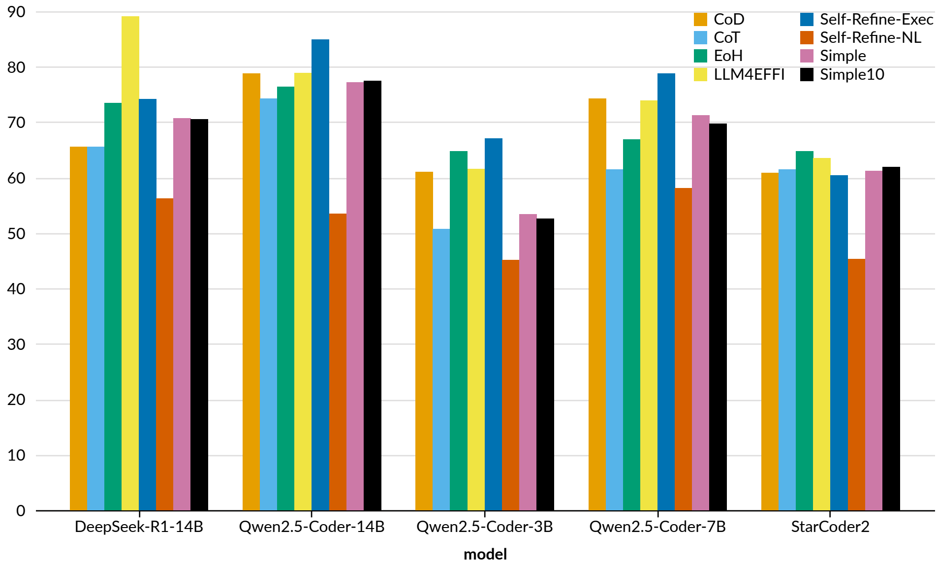
Pass@1
