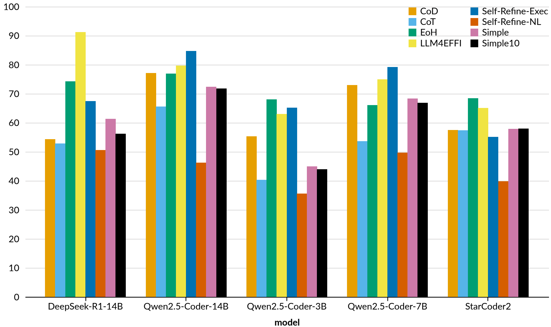
Pass@1
