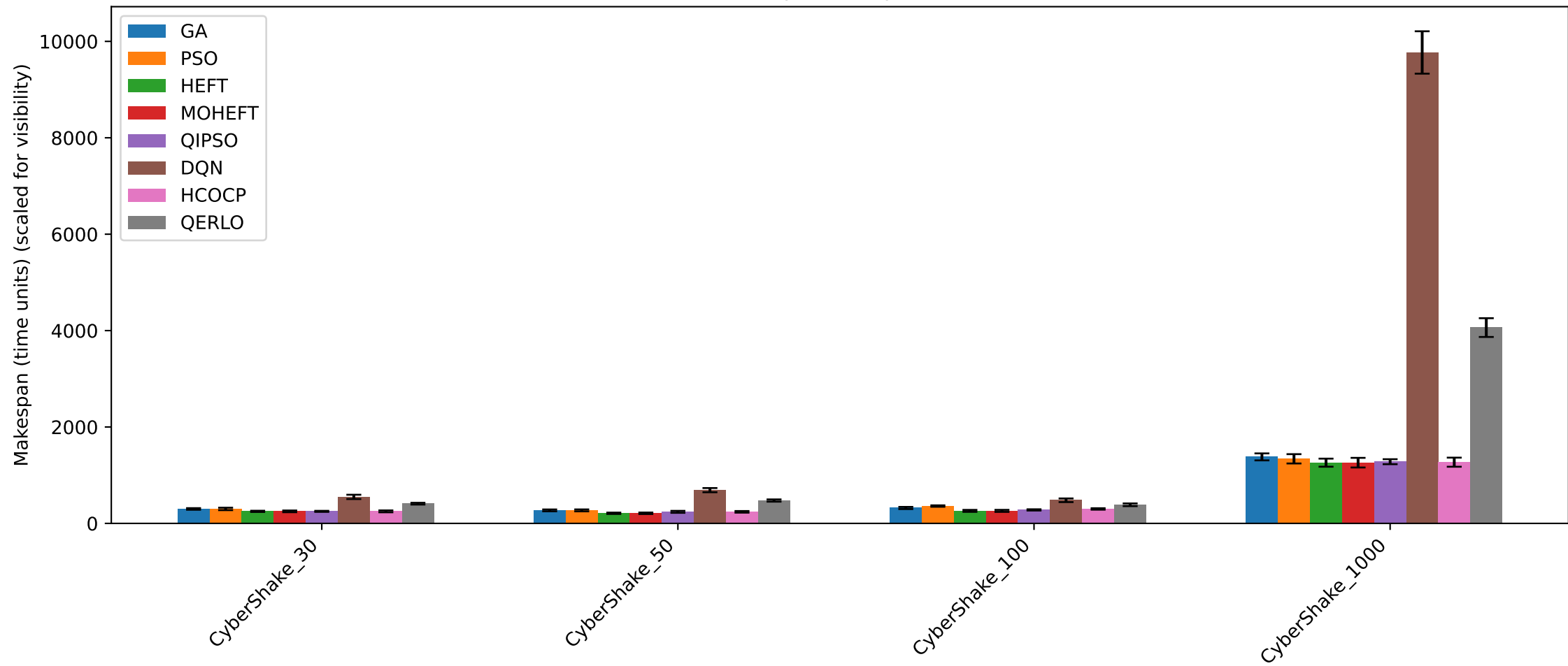
Makespan Comparison
