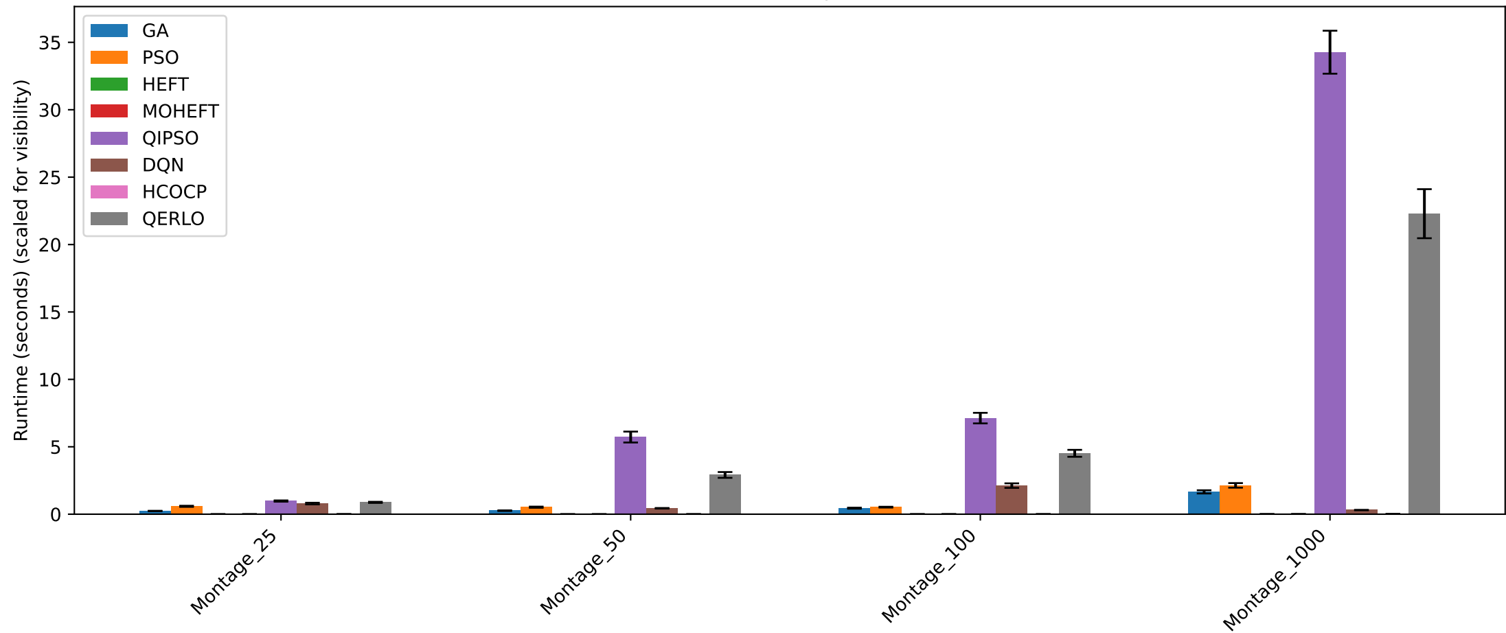
Runtime Comparison
