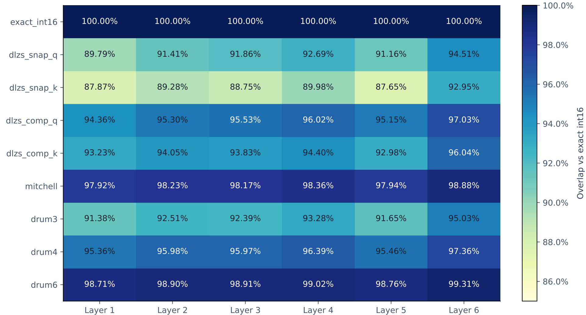
Ranking preservation by layer · 10% selection
