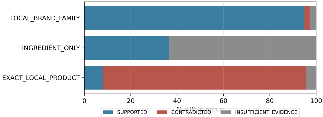
Qwen mapping assessment by pipeline resolution level
