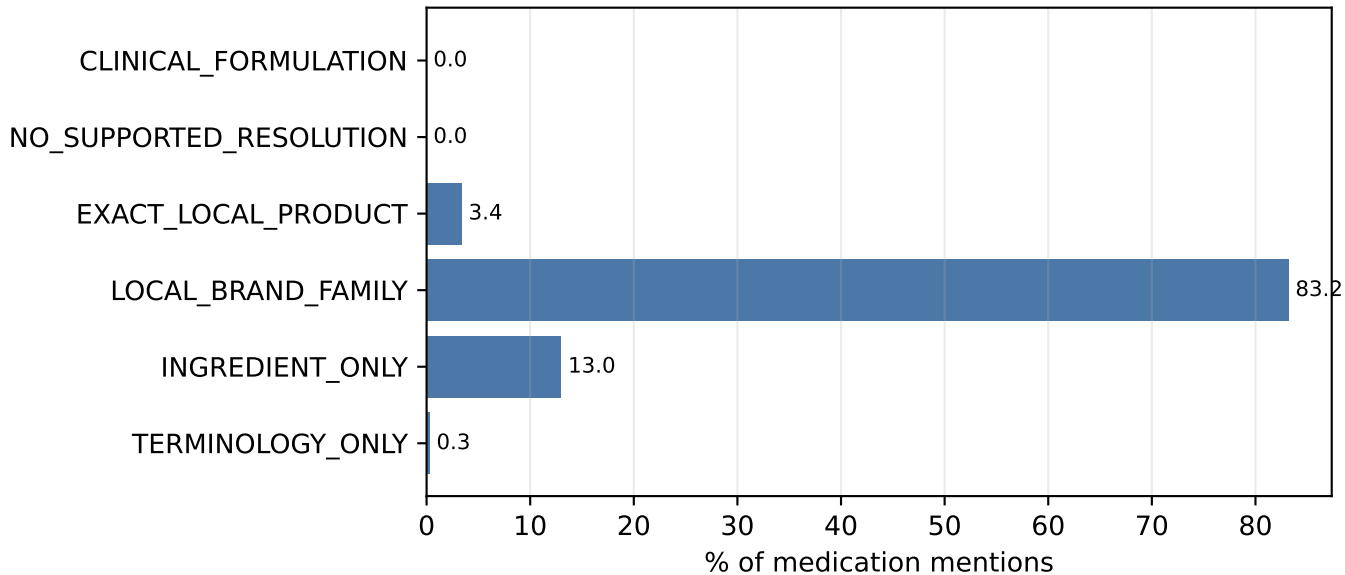
Resolution-level distribution
