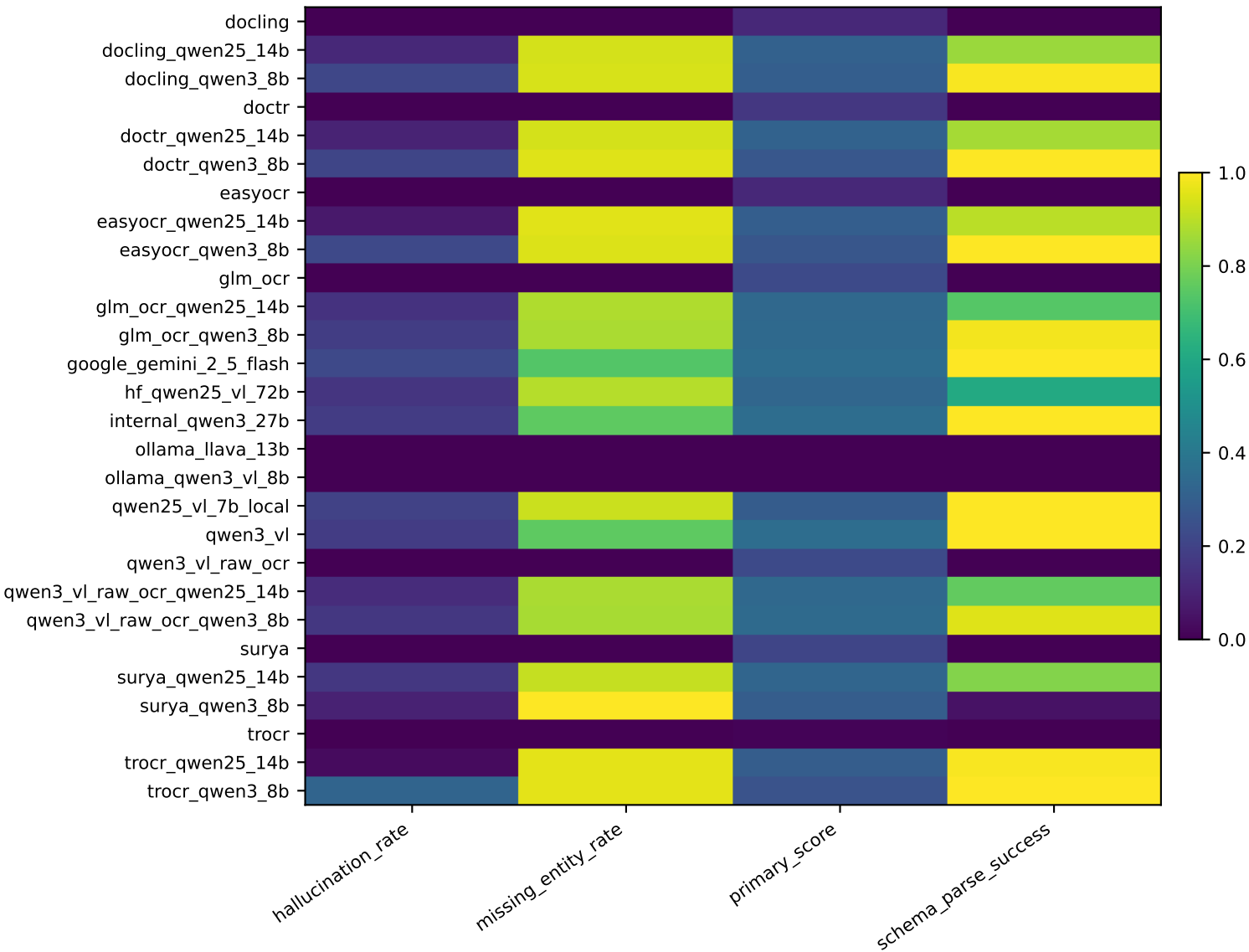
Models x Metrics Heatmap
