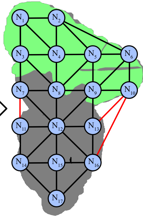
Graph construction with segmentation mask
