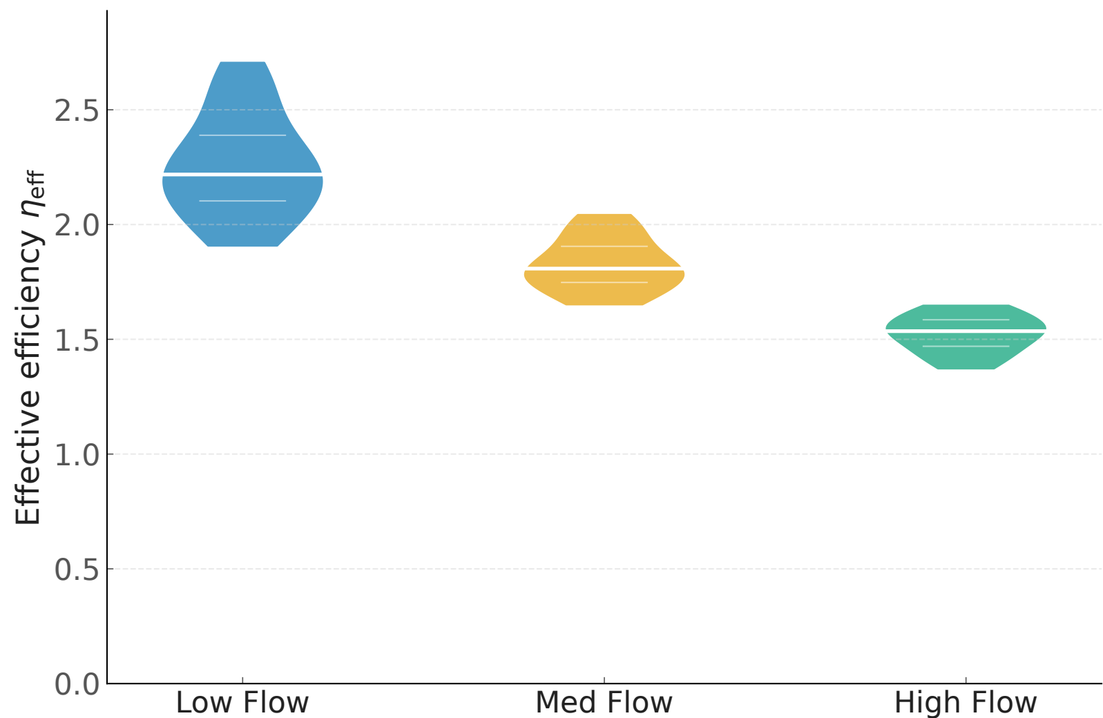
Effective efficiency distribution by fuel-flow regime — Layer 4 architecture-space sweep
