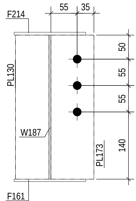
SEC A 1:5
