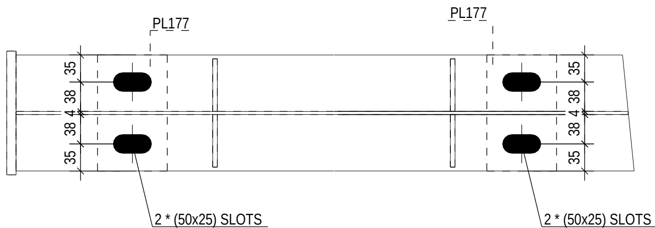
SEC A 1:5
