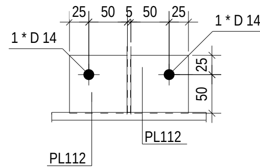
SEC A 1:5
