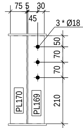
SEC A 1:10
