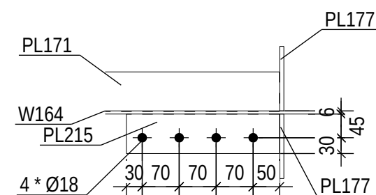
SEC B 1:10
