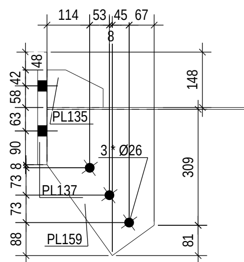
SEC A 1:10
