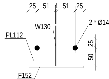
SEC A 1:5
