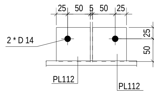
SEC A 1:5
