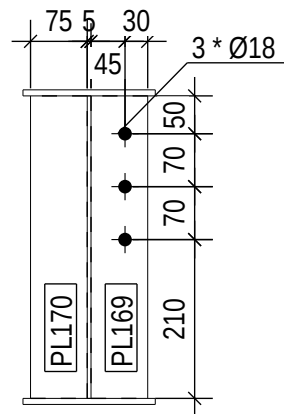
SEC A 1:10
