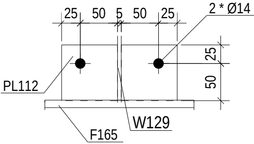
SEC A 1:5
