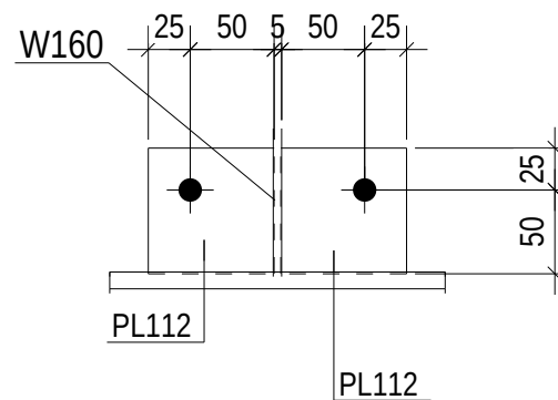
SEC A 1:5
