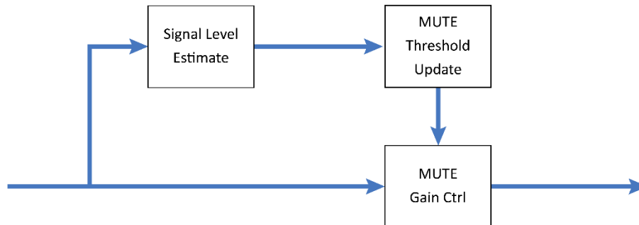
Figure 17: Auto Mute Process
