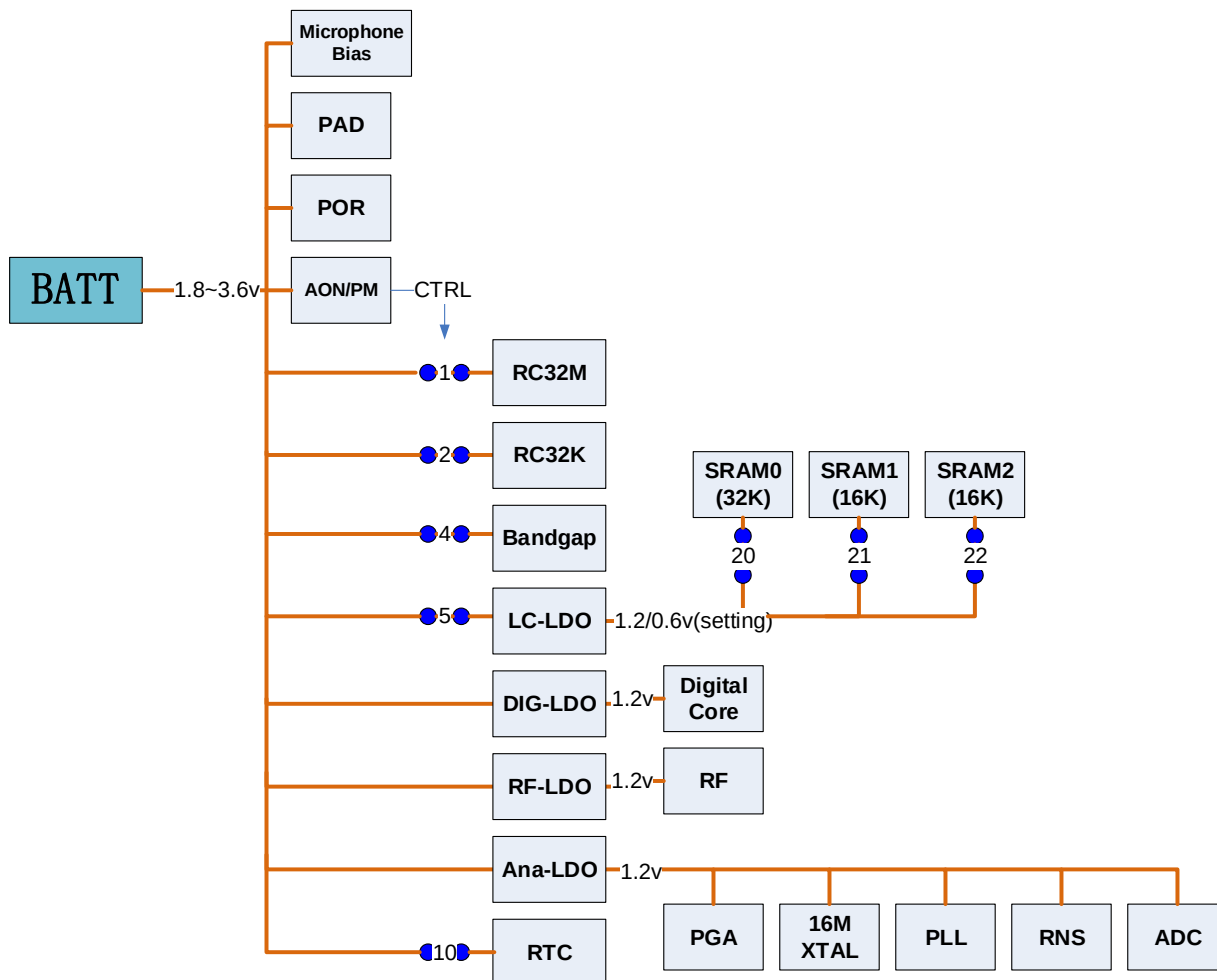
Figure 9: Power system
