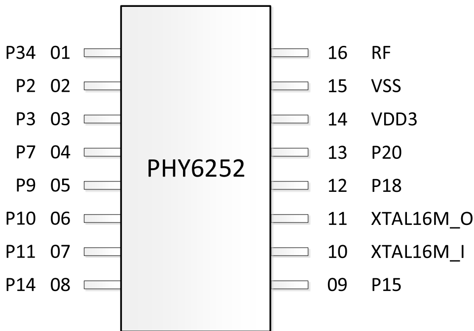
Figure 2: Pin assignment – PHY6252 TSSOP16 package
