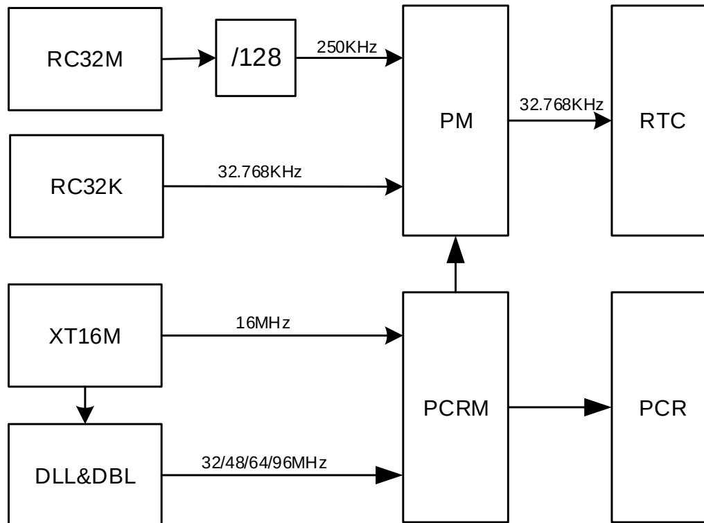
Figure 12: Clock management
