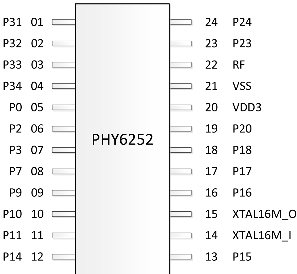
Figure 4: Pin assignment – PHY6252 SSOP24 package
