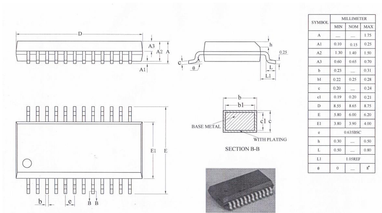
Figure 24: TSSOP24 package dimensions
