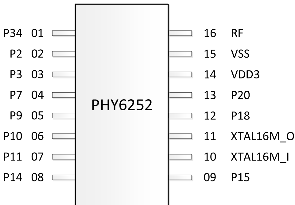
Figure 3: Pin assignment – PHY6252 SSOP16 package
