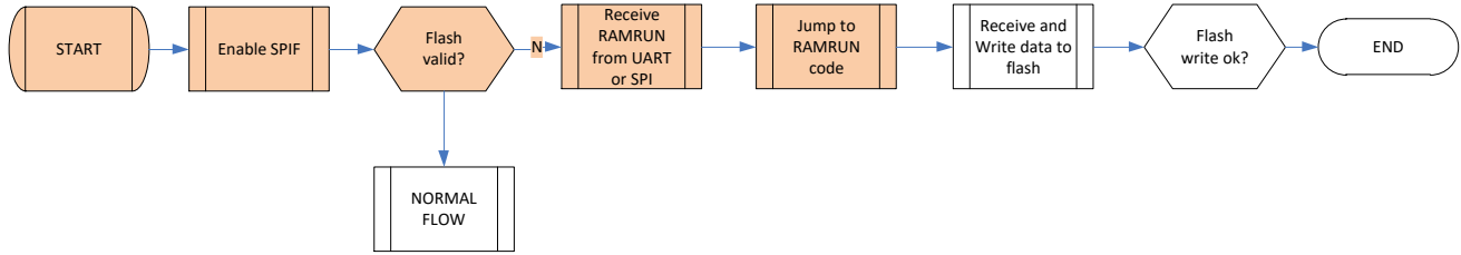
Figure 7: Bootloader flow
