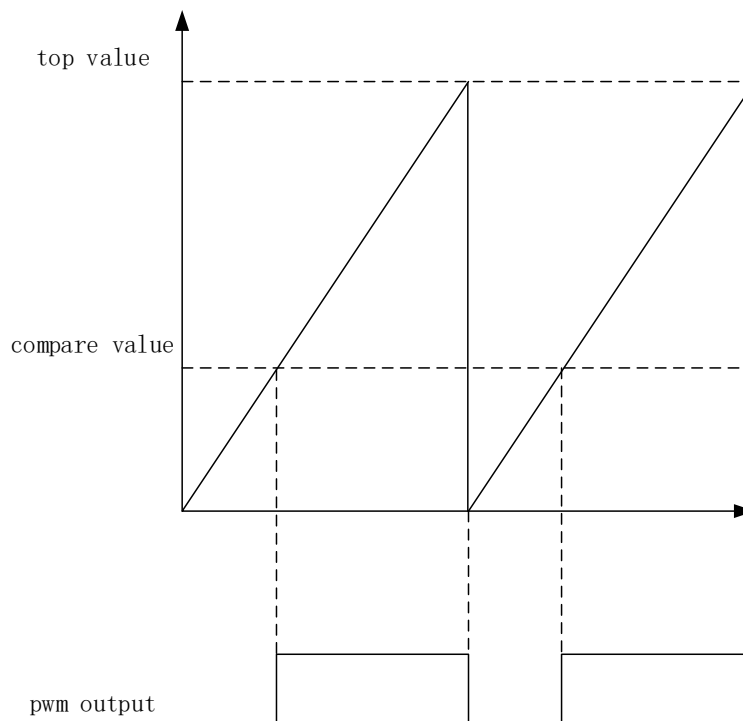
Figure 18: PWM operation
