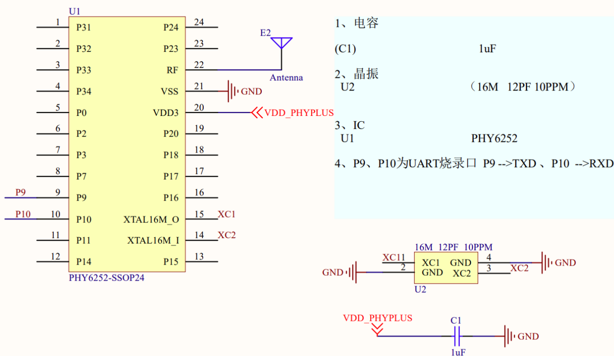
Figure 27: Sample application of SSOP24
