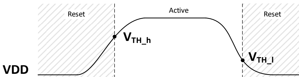
Figure 10: UVLO reset
