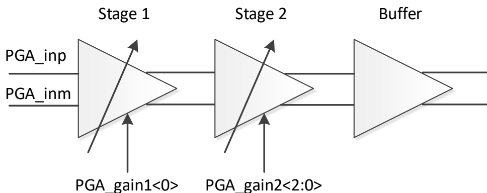
Figure 20: PGA path
