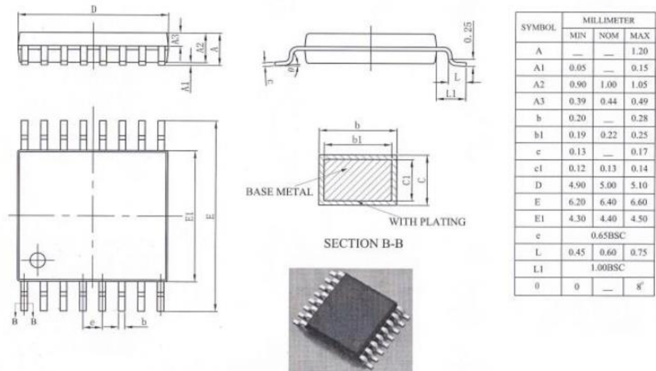
Figure 22: TSSOP16 package dimensions
