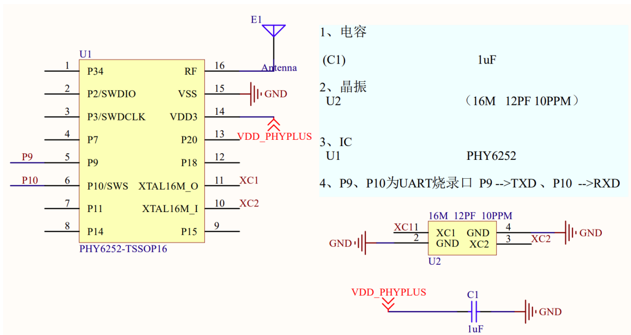
Figure 25: Sample application of TSSOP16
