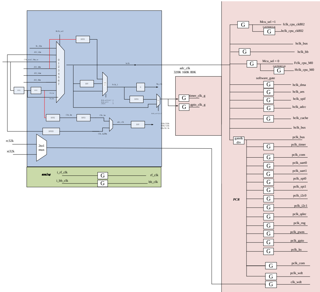
Figure 13: Clock structure diagram
