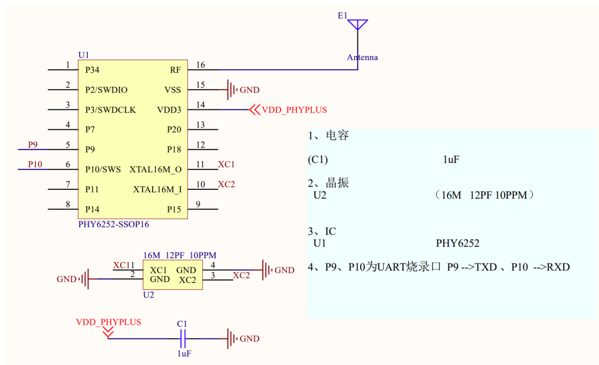
Figure 26: Sample application of SSOP16
