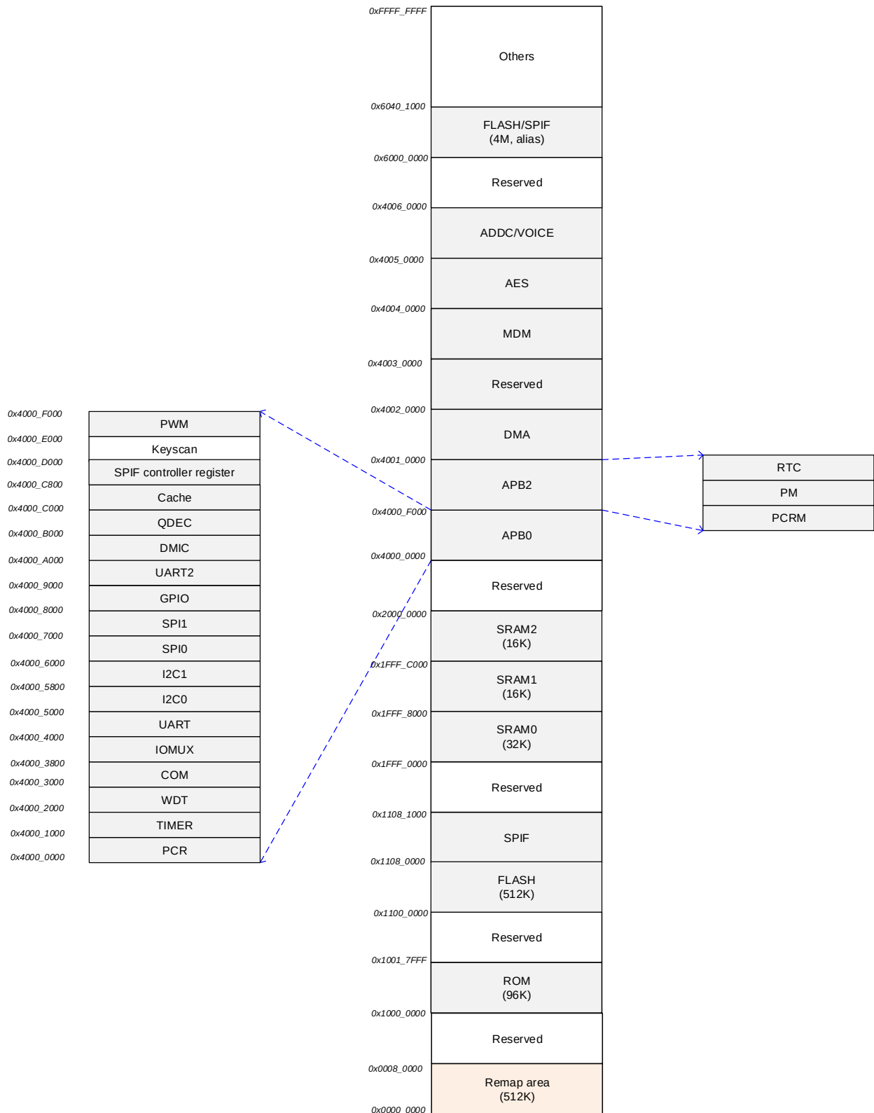
Figure 5: PHY6252 memory space
