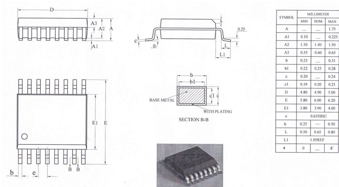
Figure 23: SSOP16 package dimensions
