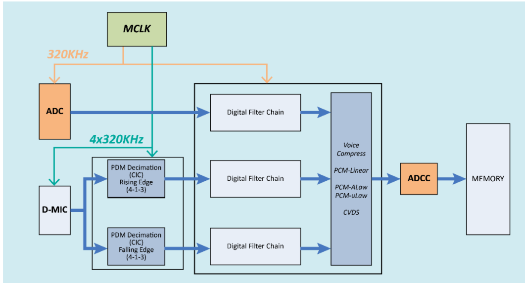
Figure 15: Block Diagram of Voice In Interface
