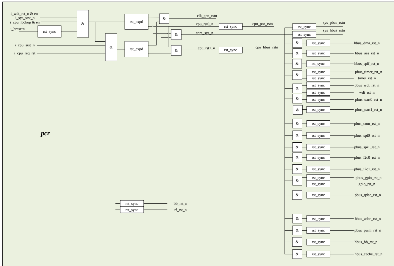
Figure 8: PHY6252 power, clock and reset
