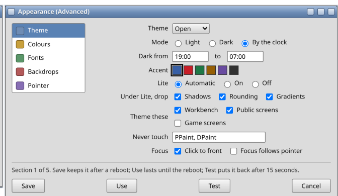
Appearance, Advanced, Theme section: every Look setting, including Lite and the never-touch list.
