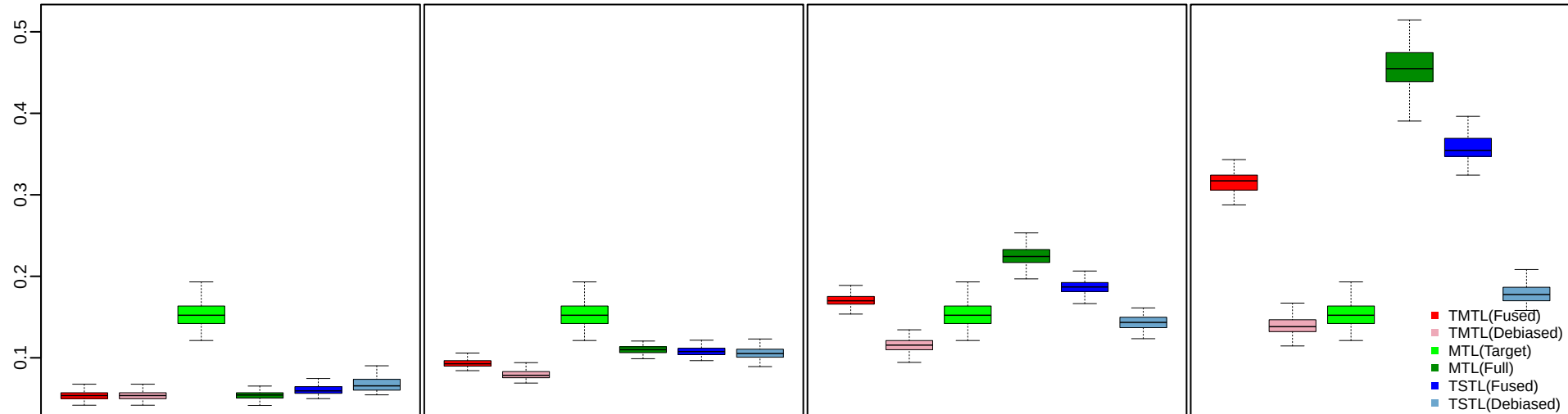
Balanced shifts
