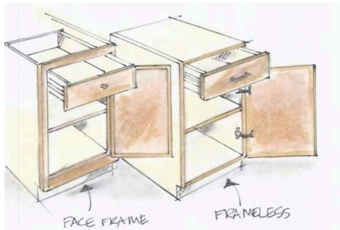
Face frame, left · frameless, right. Note what the frame does to the opening
