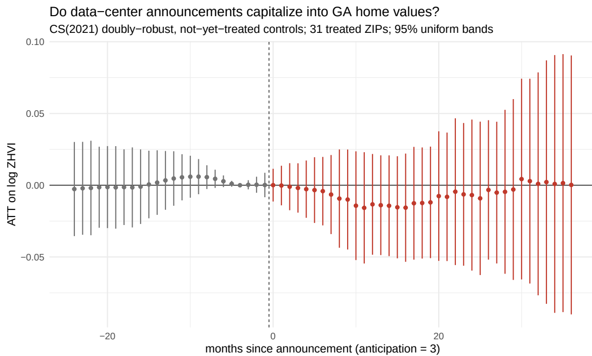
Figure 1: Event-study path of announcement effects
