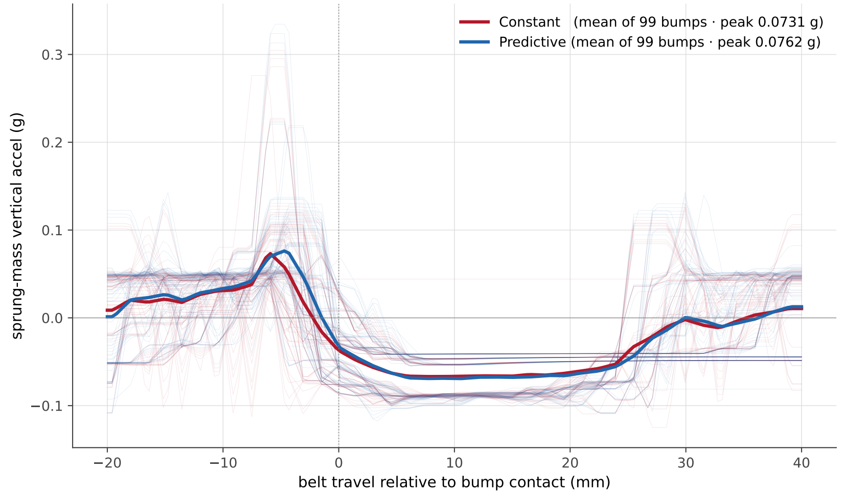
DIAG Experiment A — representative bump · Simulating · belt 0.15 m/s · mean-bump peak -4.16% Representative bump — ensemble mean (bold) over individual bumps (faint), despiked
