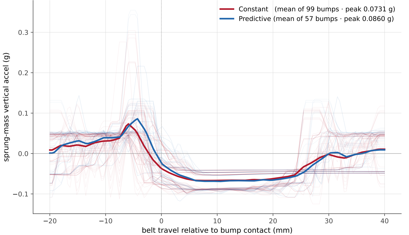
DIAG Experiment A — representative bump · Simulating · belt 0.15 m/s · mean-bump peak -17.56% Representative bump — ensemble mean (bold) over individual bumps (faint), despiked
