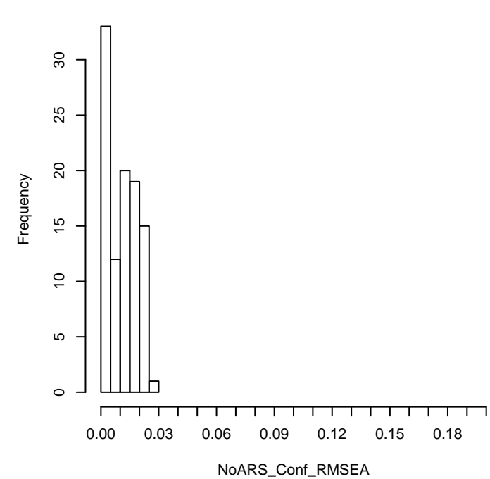
N = 250, ARS = 0.3, Nfac = 2, scale = unbalanced
