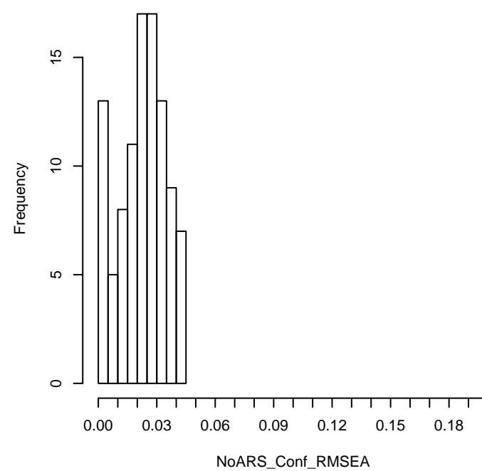
N = 250, ARS = 0.6, Nfac = 2, scale = semi-balanced
