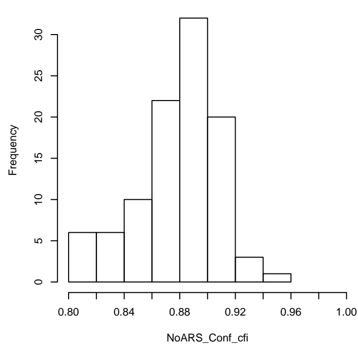
N = 250, ARS = 0.6, Nfac = 2, scale = semi-balanced
