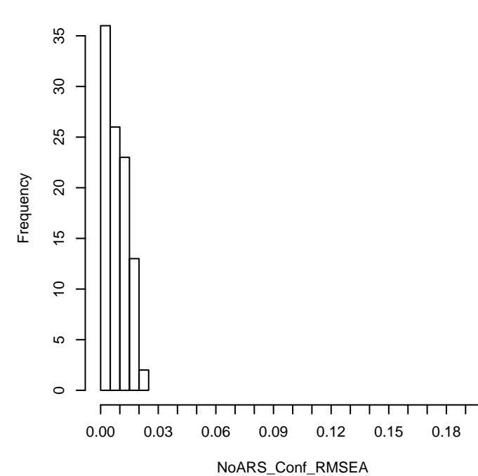
N = 1000, ARS = 0.6, Nfac = 2, scale = unbalanced
