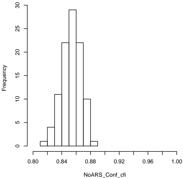
N = 1000, ARS = 0.6, Nfac = 2, scale = balanced
