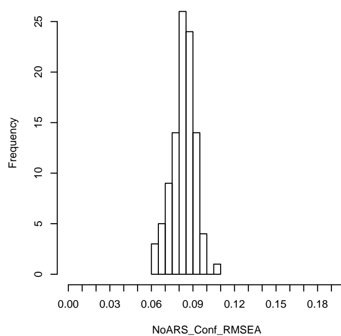
N = 250, ARS = 0.6, Nfac = 2, scale = semi-balanced
