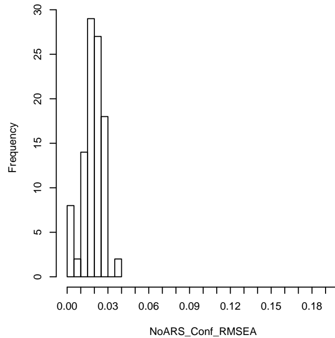
N = 250, ARS = 0.3, Nfac = 2, scale = semi-balanced
