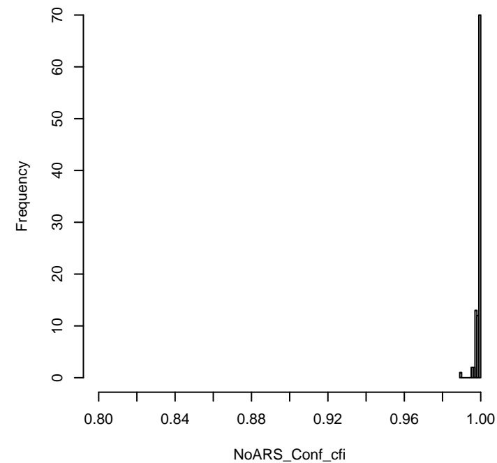
N = 1000, ARS = 0.6, Nfac = 2, scale = unbalanced
