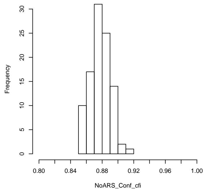
N = 1000, ARS = 0.6, Nfac = 2, scale = semi-balanced
