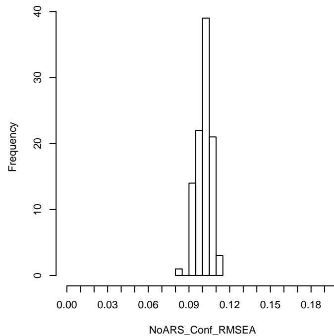
N = 1000, ARS = 0.6, Nfac = 2, scale = semi-balanced
