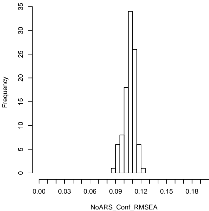
N = 1000, ARS = 0.6, Nfac = 2, scale = balanced
