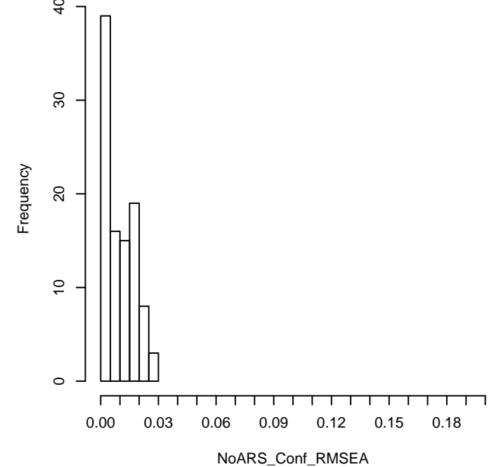
N = 250, ARS = 0.6, Nfac = 2, scale = unbalanced
