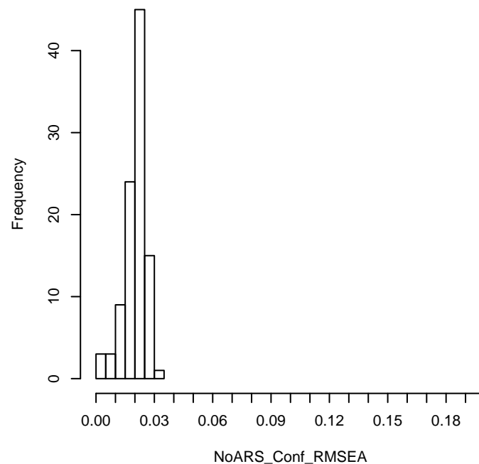
N = 1000, ARS = 0.6, Nfac = 2, scale = semi-balanced
