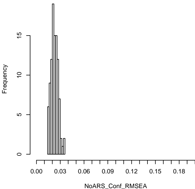
N = 1000, ARS = 0.6, Nfac = 2, scale = balanced
