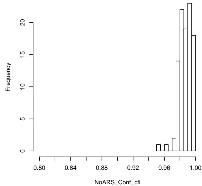
N = 250, ARS = 0.6, Nfac = 2, scale = semi-balanced
