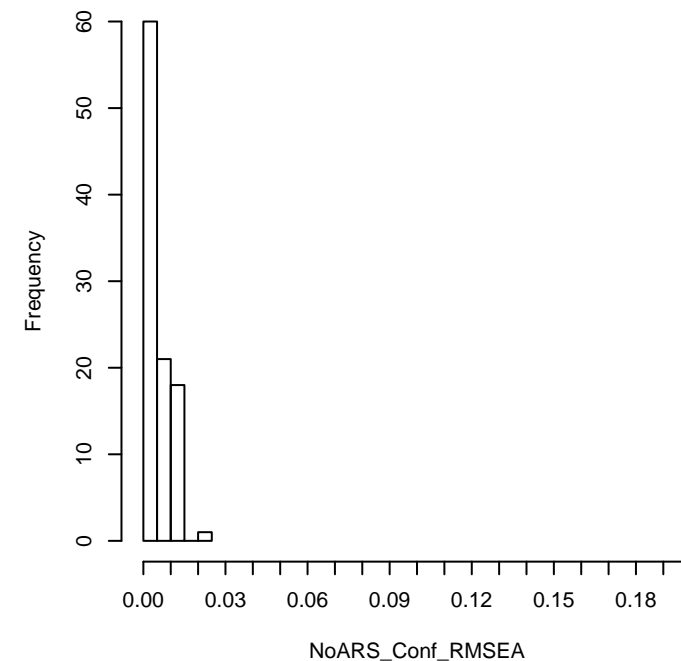
N = 1000, ARS = 0.6, Nfac = 2, scale = unbalanced
