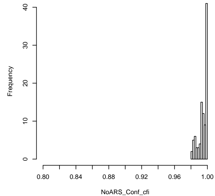
N = 250, ARS = 0.6, Nfac = 2, scale = unbalanced
