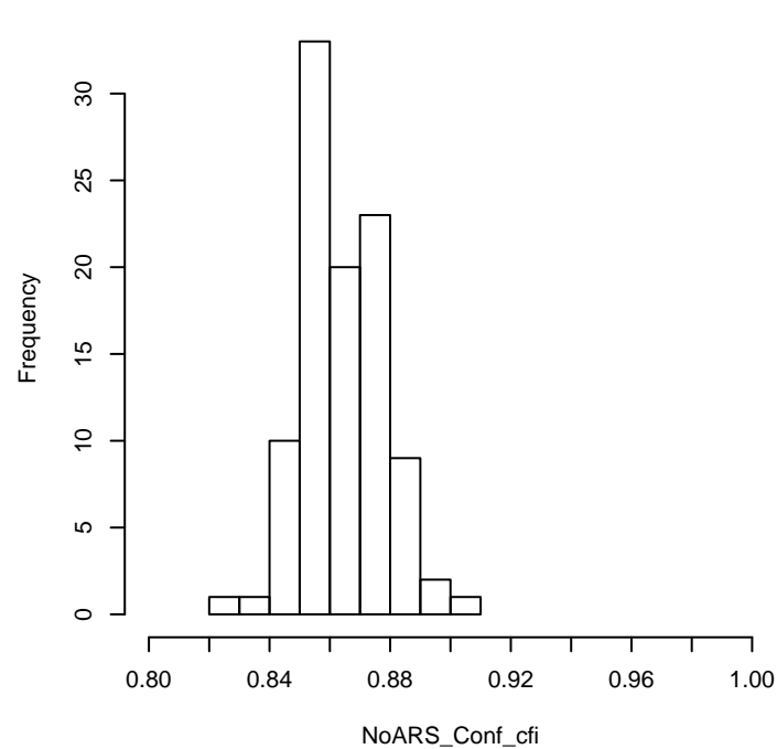
N = 1000, ARS = 0.6, Nfac = 2, scale = semi-balanced
