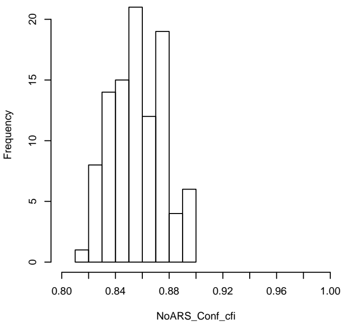
N = 1000, ARS = 0.6, Nfac = 2, scale = balanced
