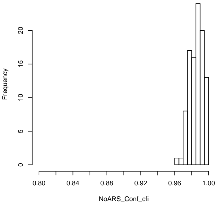
N = 250, ARS = 0.6, Nfac = 2, scale = balanced
