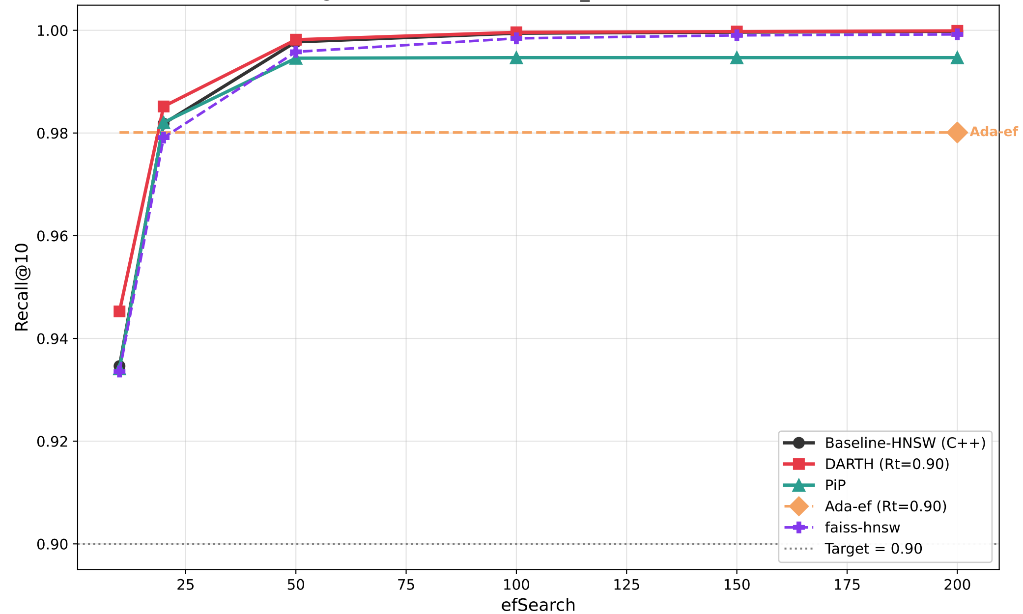
Recall@10 vs efSearch — fashion_mnist (M=16, efC=128)
