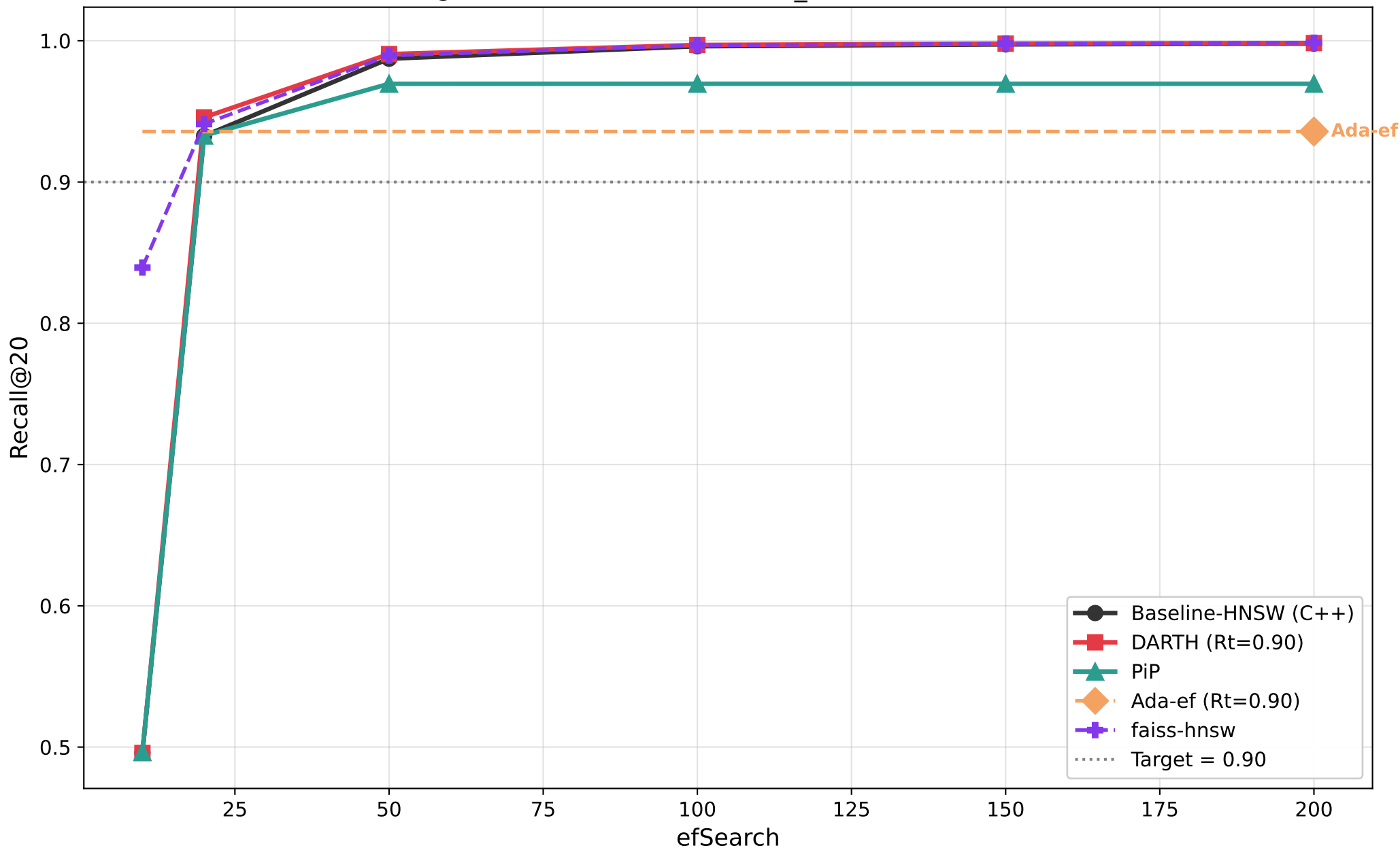
Recall@20 vs efSearch — fashion_mnist (M=8, efC=200)
