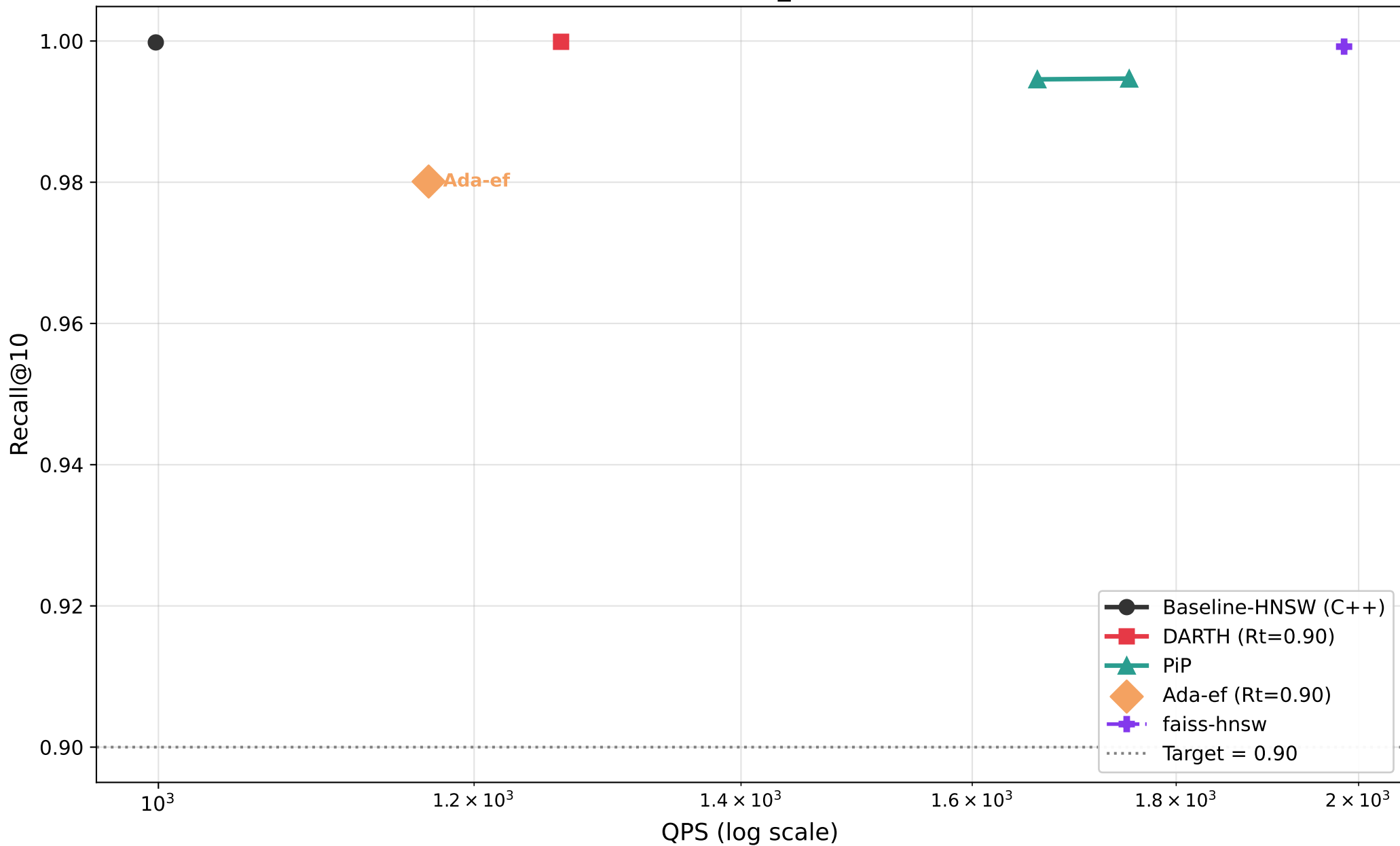
Recall@10 vs QPS — fashion_mnist (M=16, efC=128)
