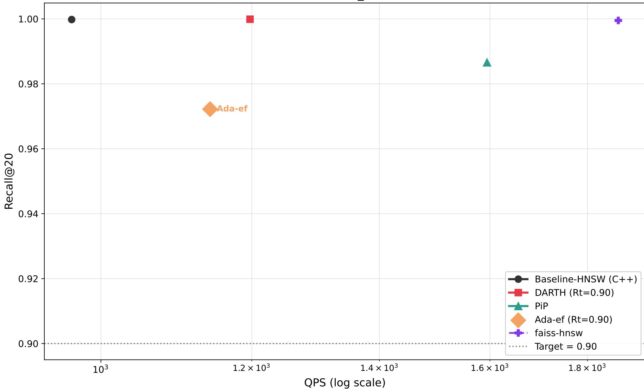
Recall@20 vs QPS — fashion_mnist (M=16, efC=200)
