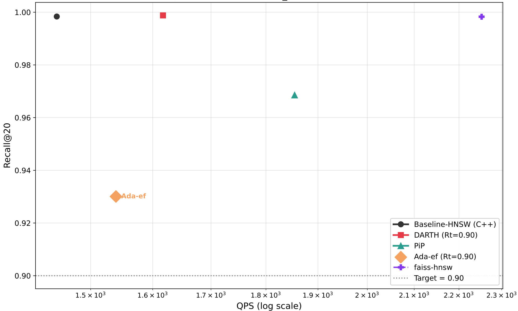
Recall@20 vs QPS — fashion_mnist (M=8, efC=128)
