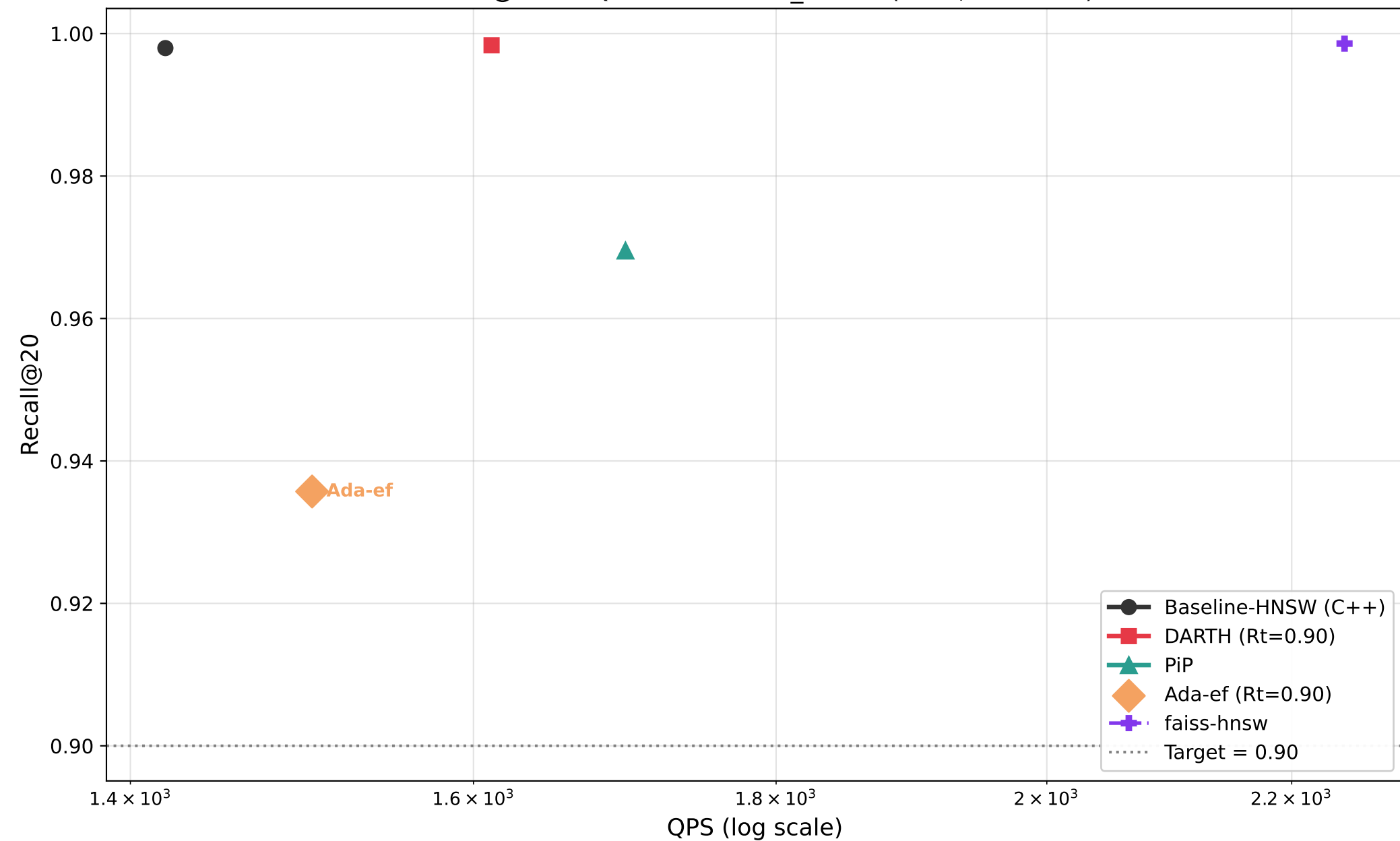
Recall@20 vs QPS — fashion_mnist (M=8, efC=200)
