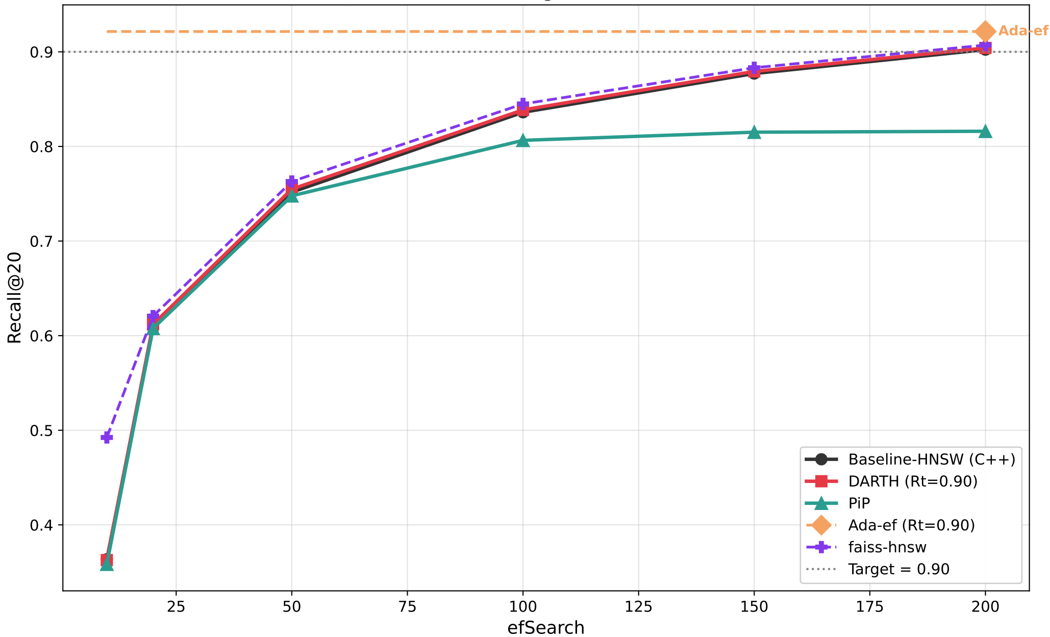
Recall@20 vs efSearch — glove100 (M=16, efC=200)
