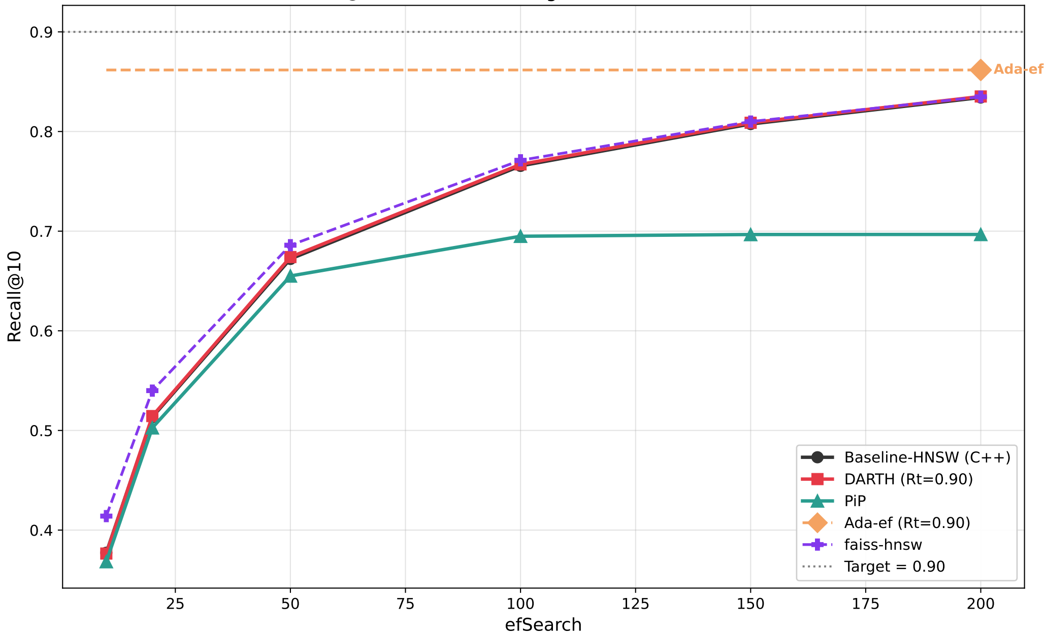
Recall@10 vs efSearch — glove100 (M=8, efC=128)
