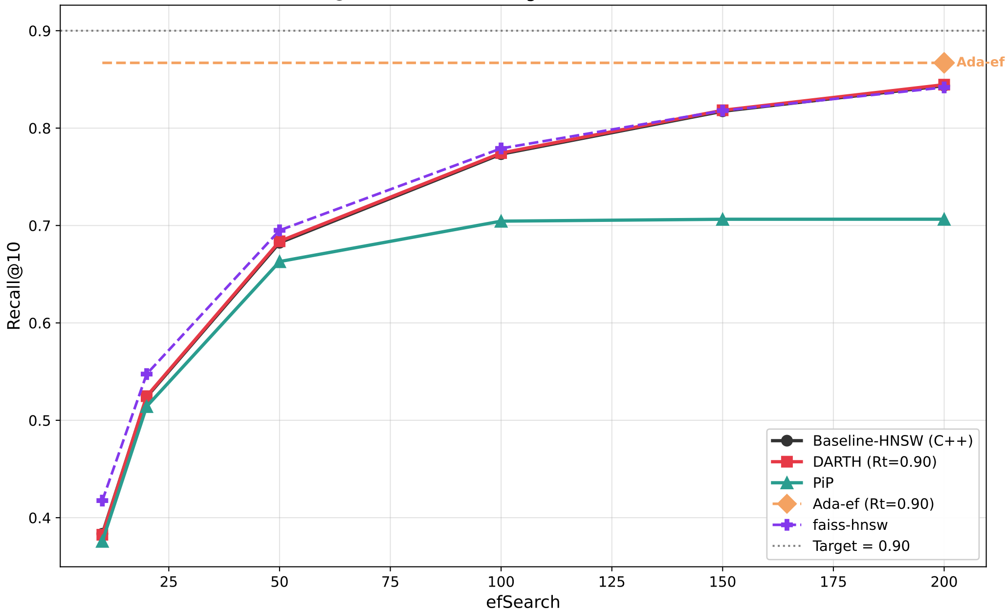
Recall@10 vs efSearch — glove100 (M=8, efC=200)
