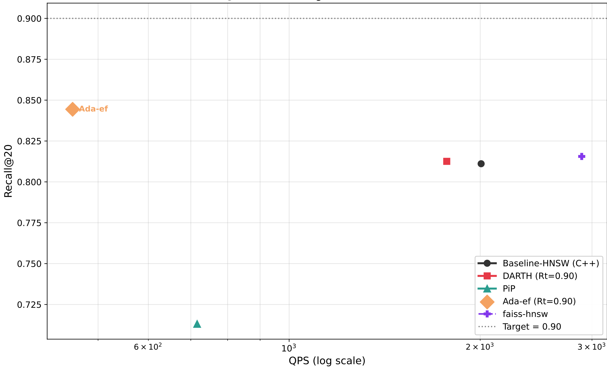
Recall@20 vs QPS — glove100 (M=8, efC=128)
