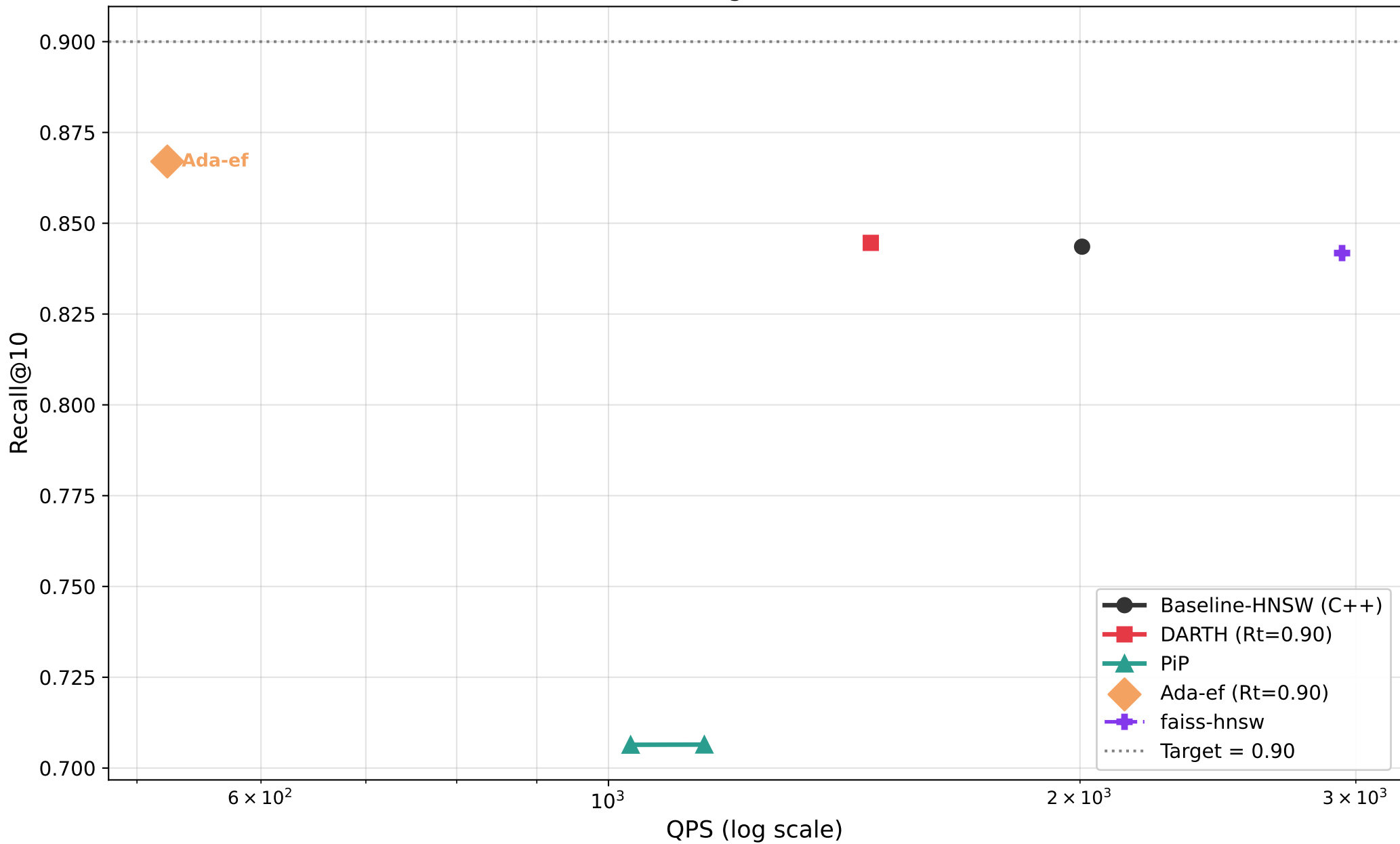
Recall@10 vs QPS — glove100 (M=8, efC=200)
