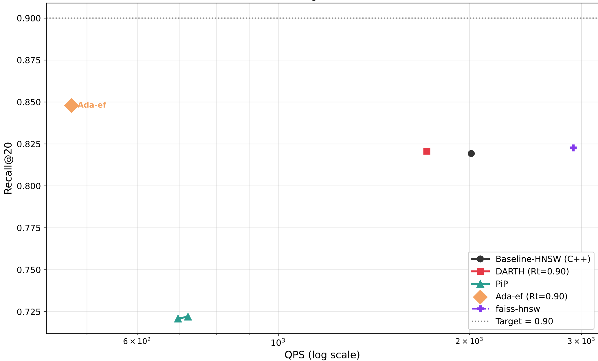
Recall@20 vs QPS — glove100 (M=8, efC=200)
