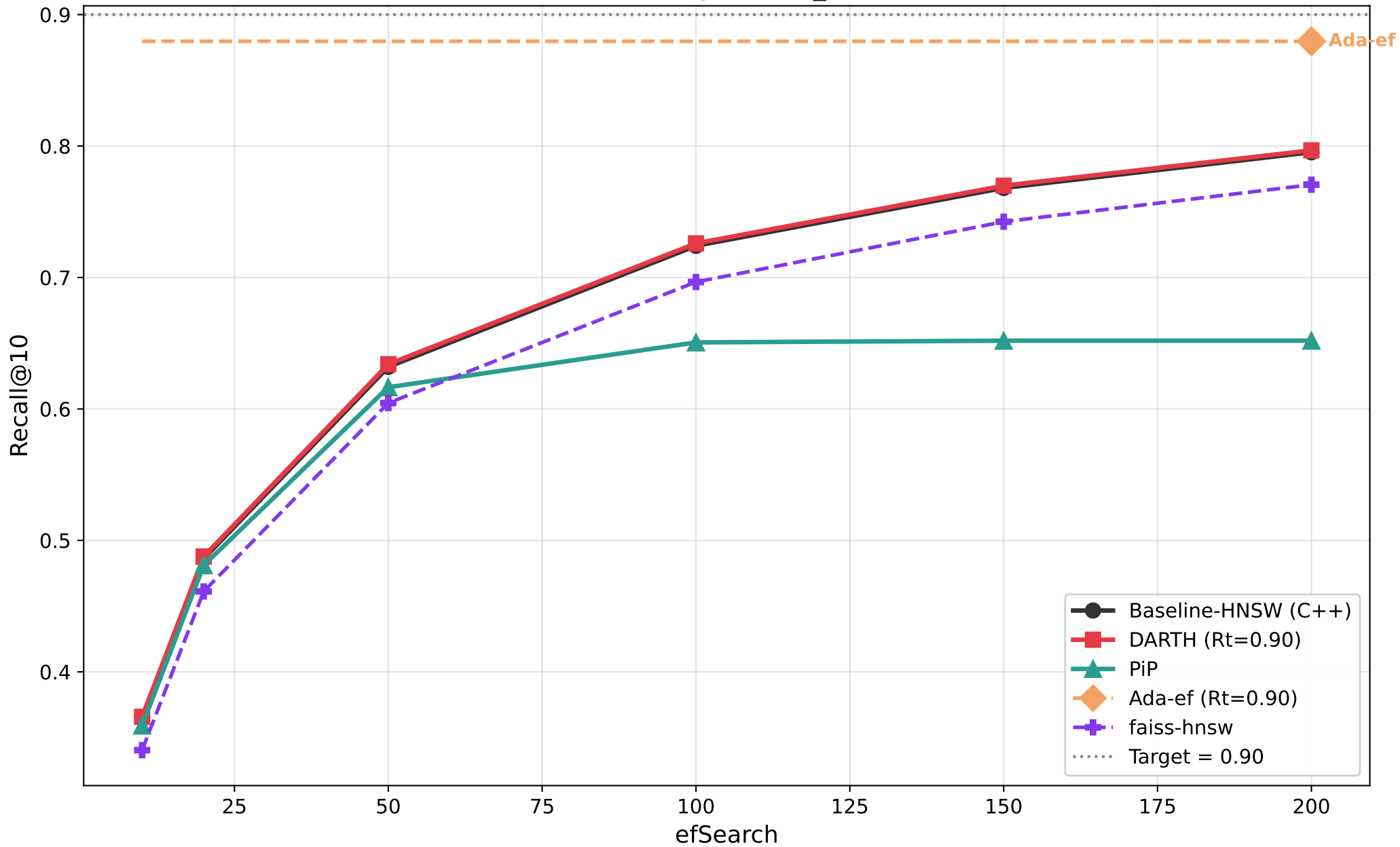
Recall@10 vs efSearch — glove100_full (M=16, efC=128)
