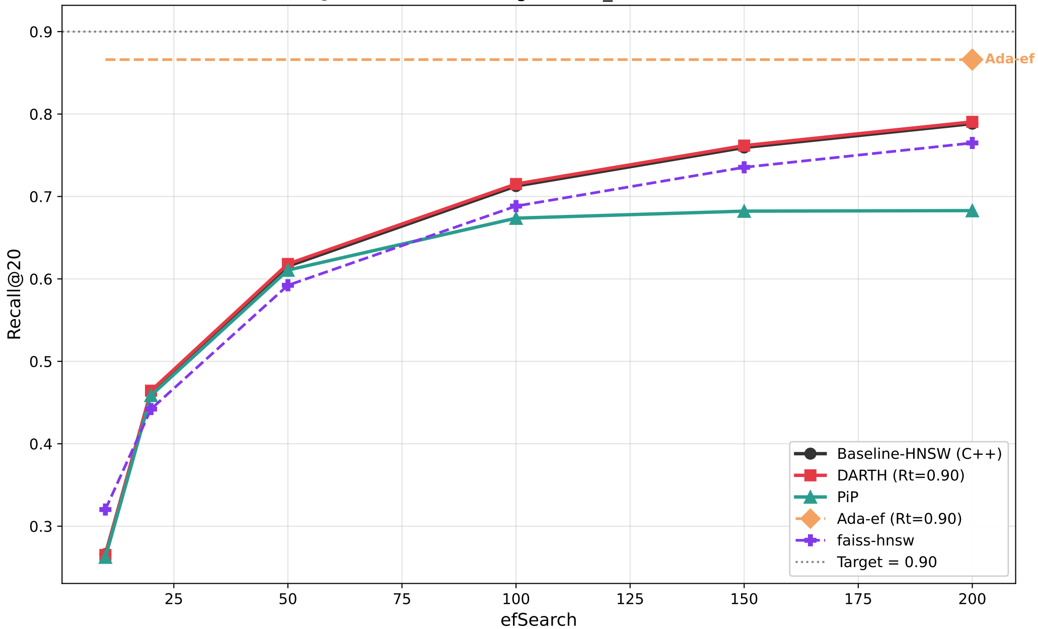
Recall@20 vs efSearch — glove100_full (M=16, efC=128)
